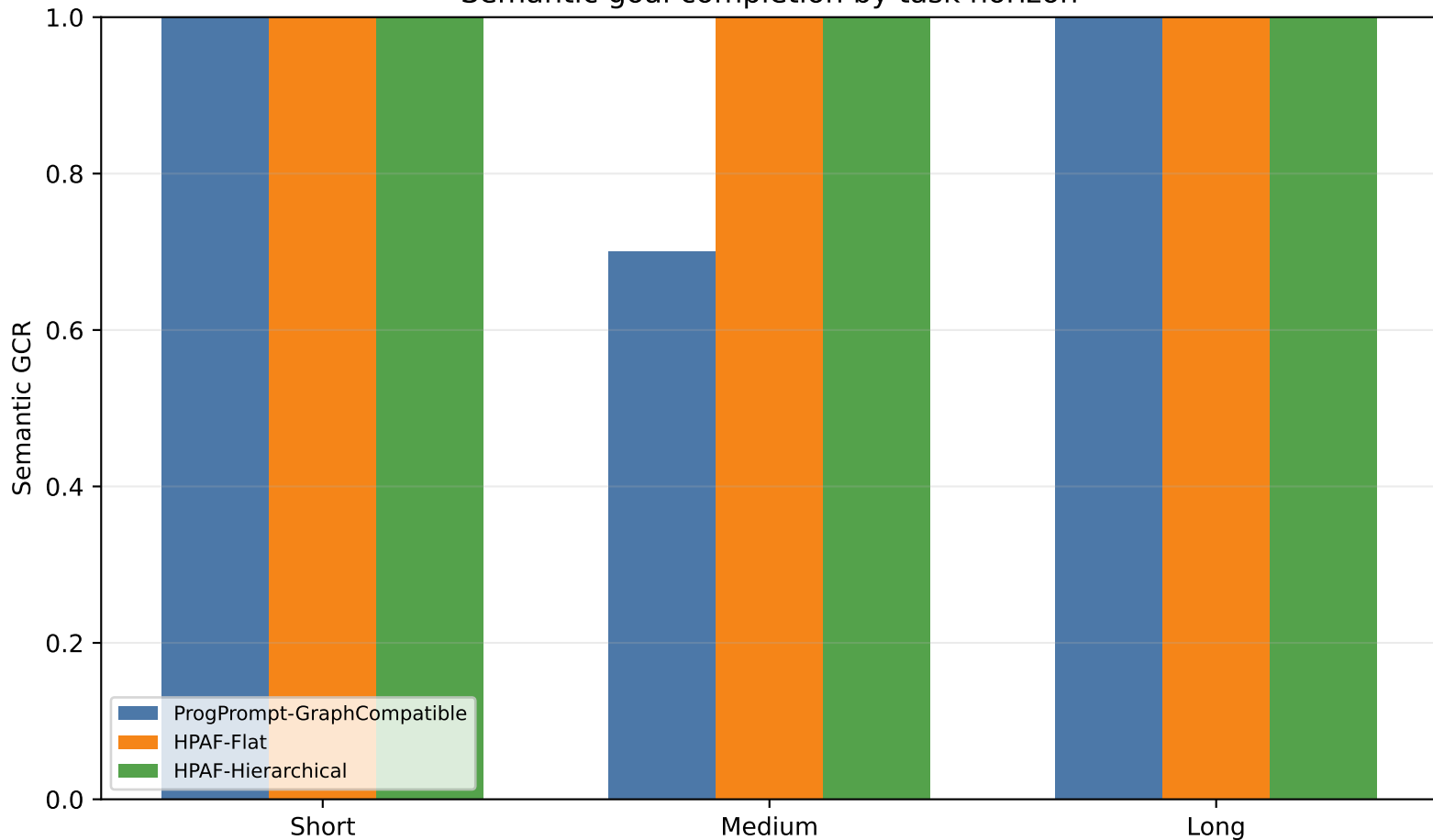
Semantic goal completion by task horizon
