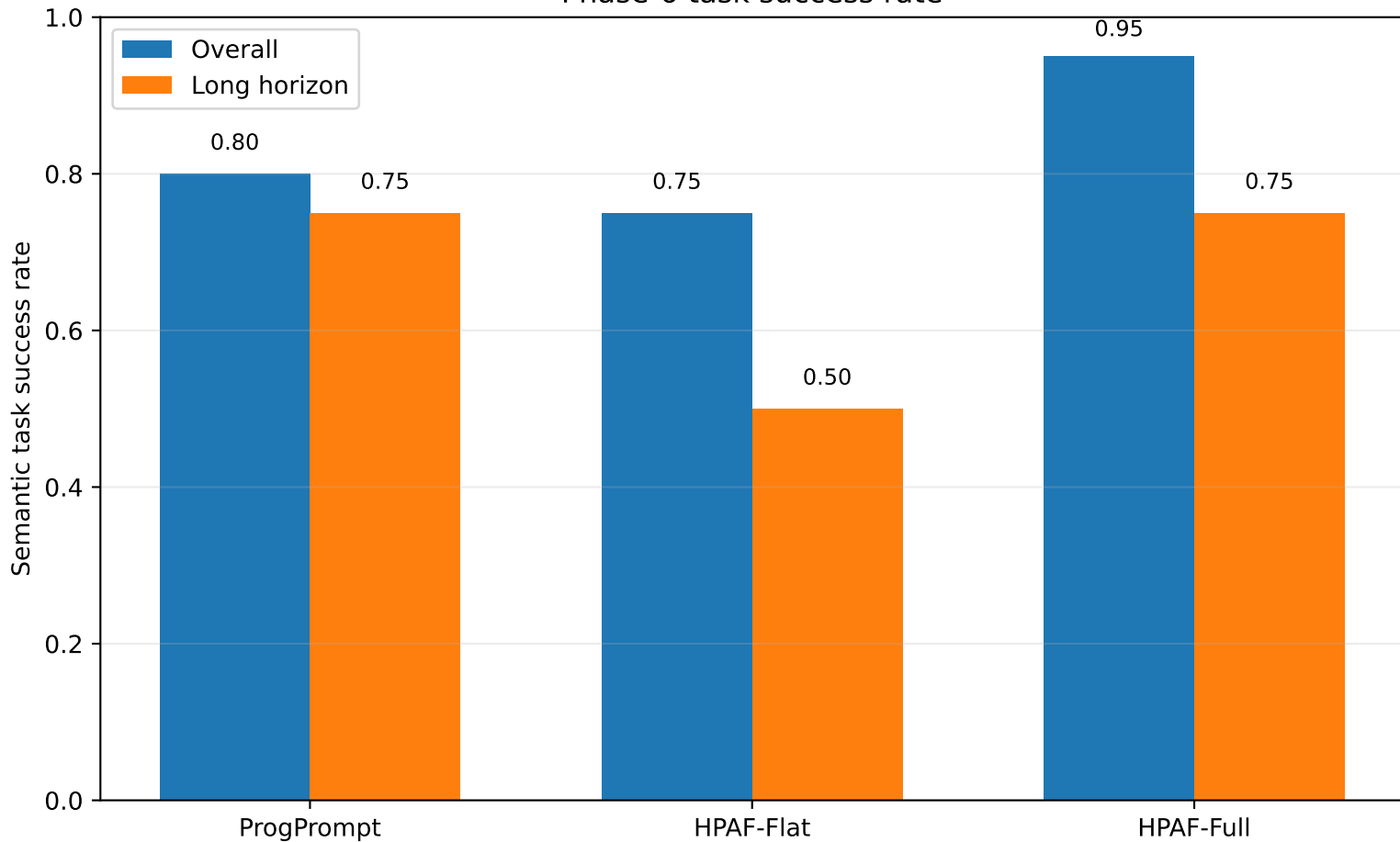
Phase-6 task success rate
