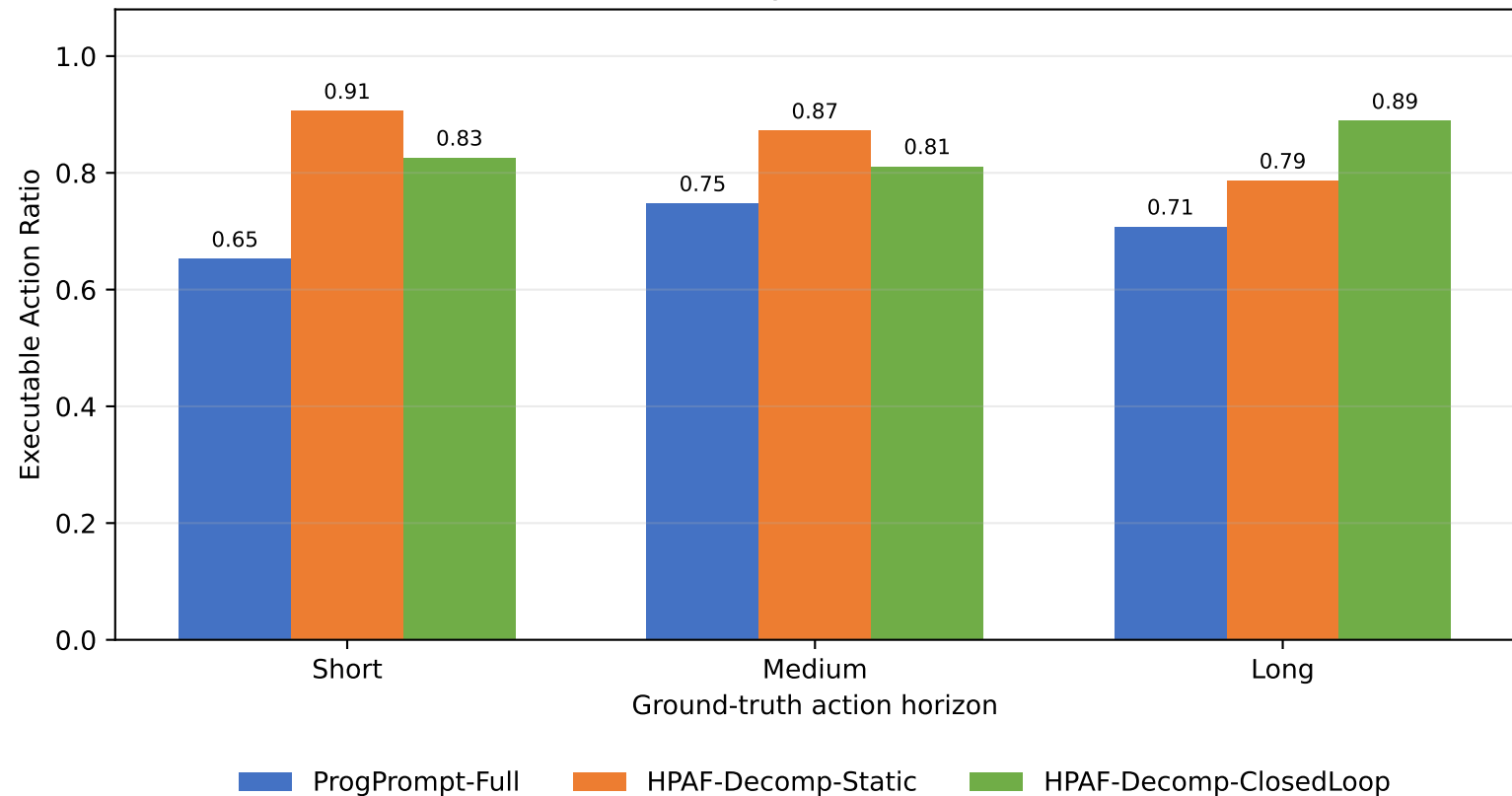
Executability vs Task Horizon
