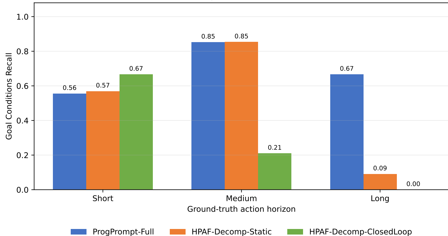
Goal Completion vs Task Horizon
