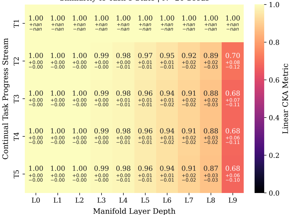
Bootstrapped Temporal CKA Stability ( \alpha=2.0 , g=1.0 ) Similarity to Task 1 State | N=20 Seeds
