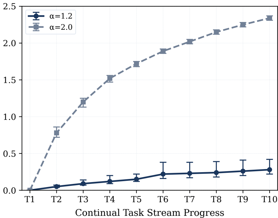
Distance From Task 1 Subspace
