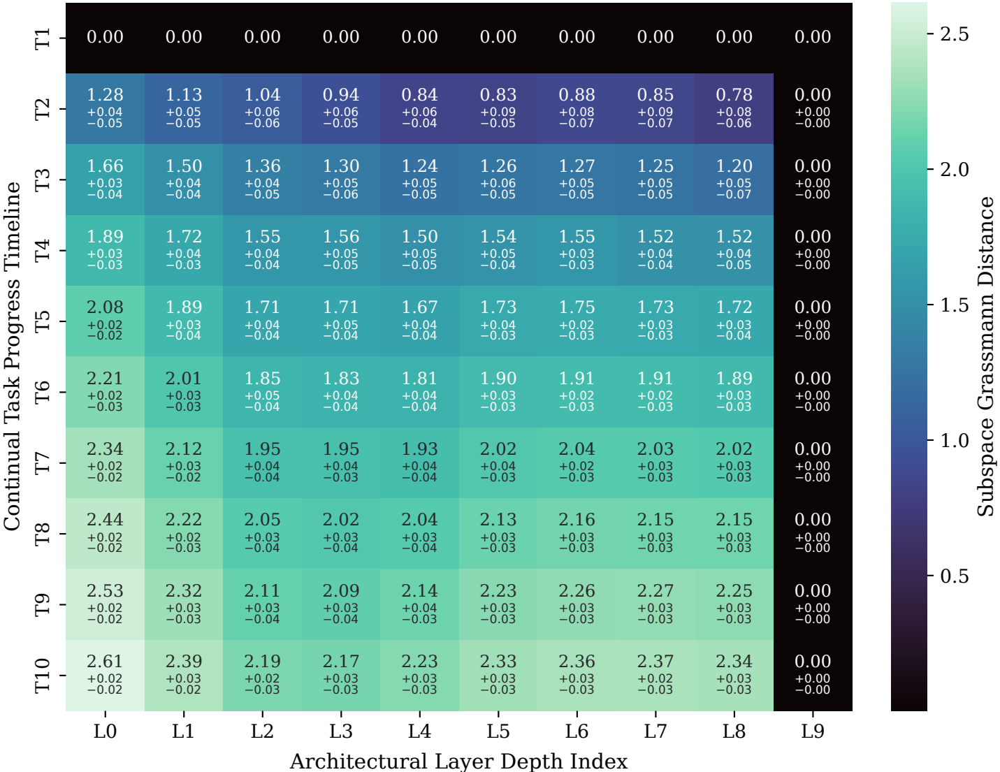
Bootstrapped Weight Subspace Rotation ( \alpha=2.0 , g=1.0 ) Grassmann Distance to Task 1 Baseline | N=20 Seeds
