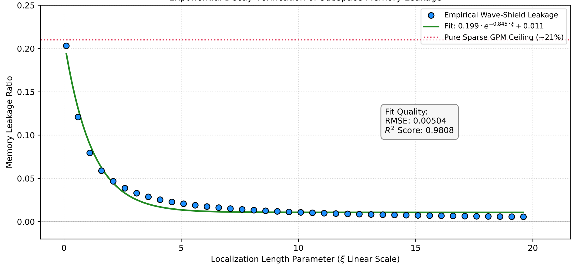
Exponential Decay Verification of Subspace Memory Leakage
