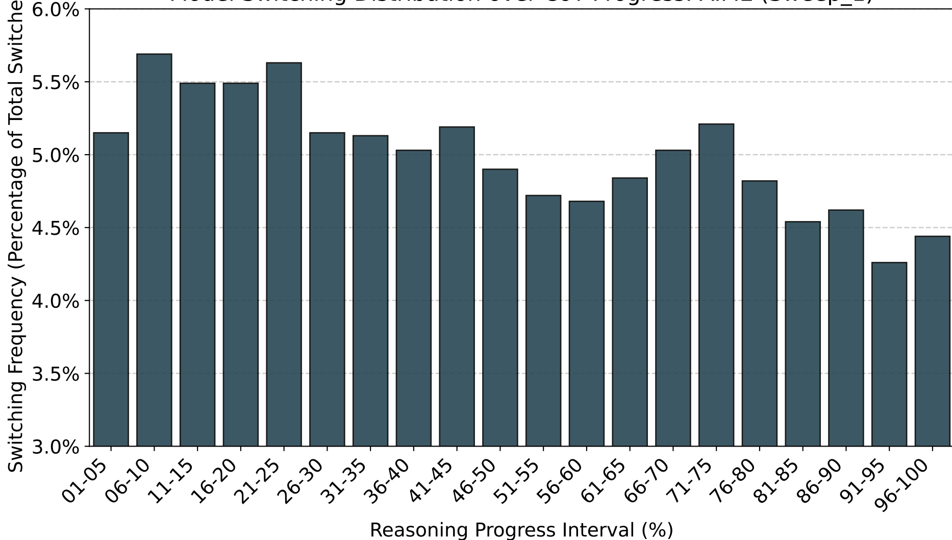
Model Switching Distribution over CoT Progress: AIME (Sweep_1)
