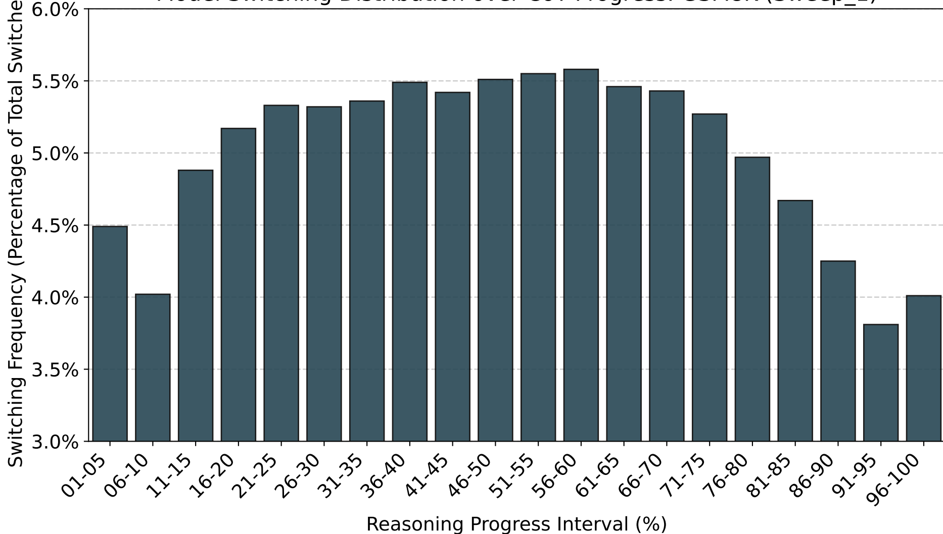
Model Switching Distribution over CoT Progress: GSM8K (Sweep_1)
