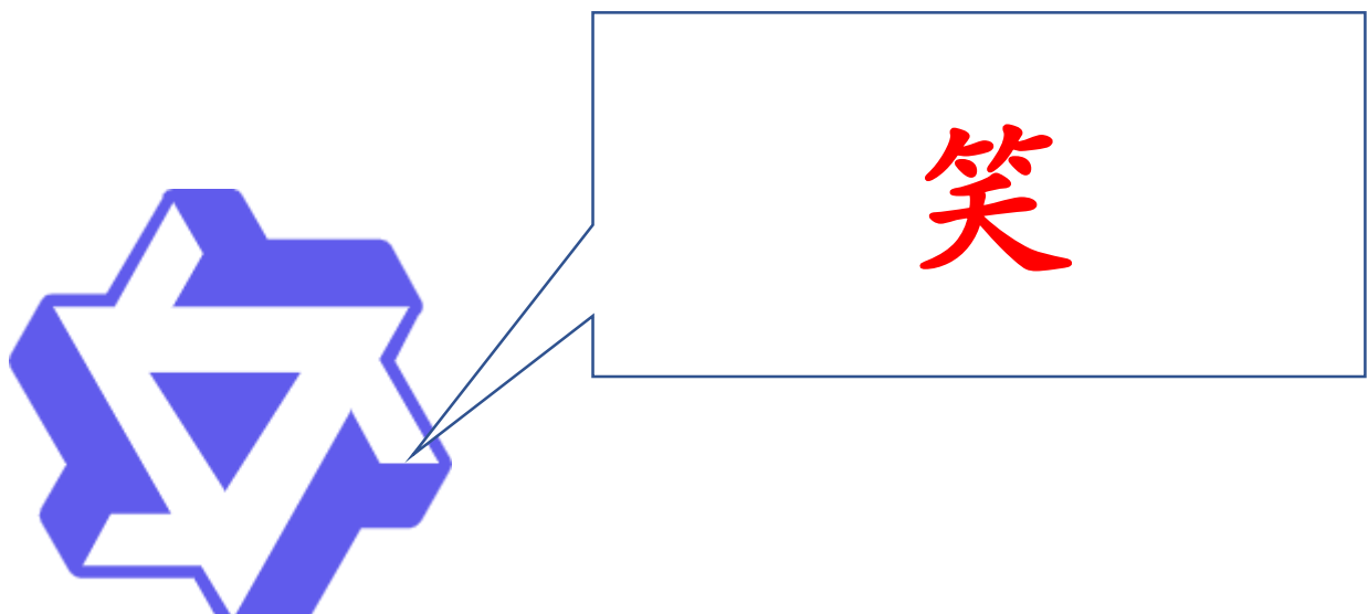
Qwen-VL-Max
