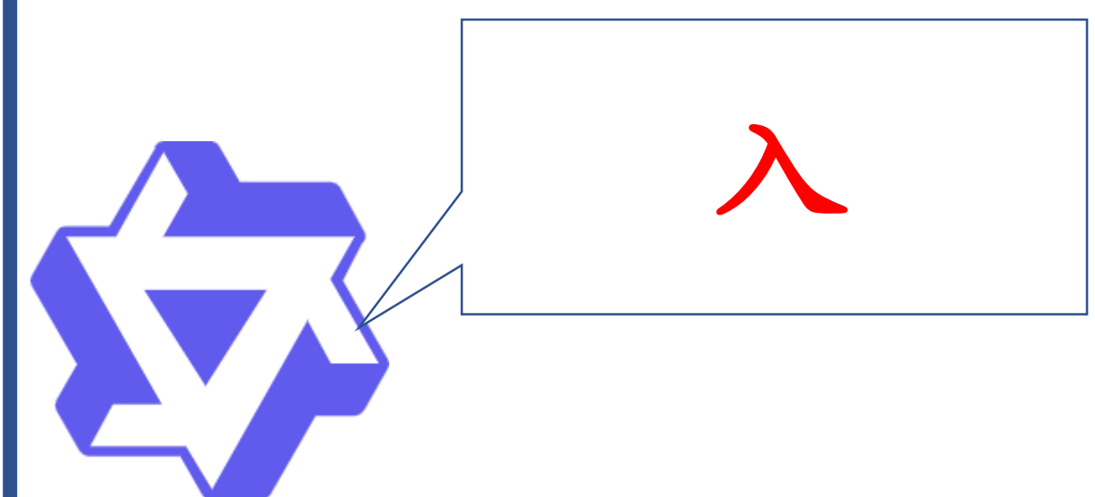
Qwen-VL-Max
