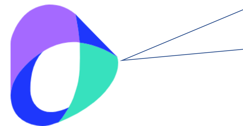
Seed-1.6-VL
