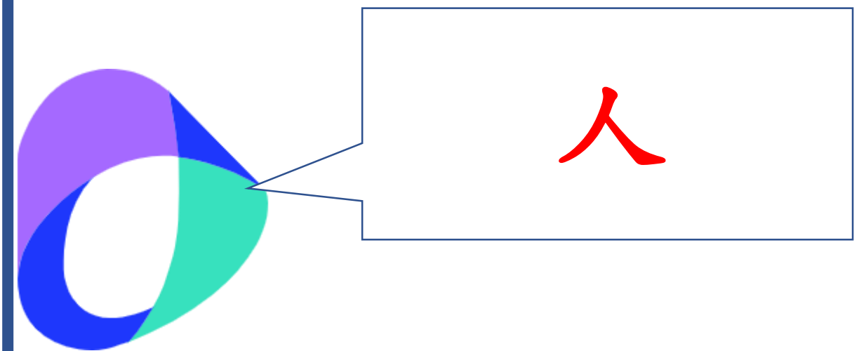
Seed-1.6-VL
