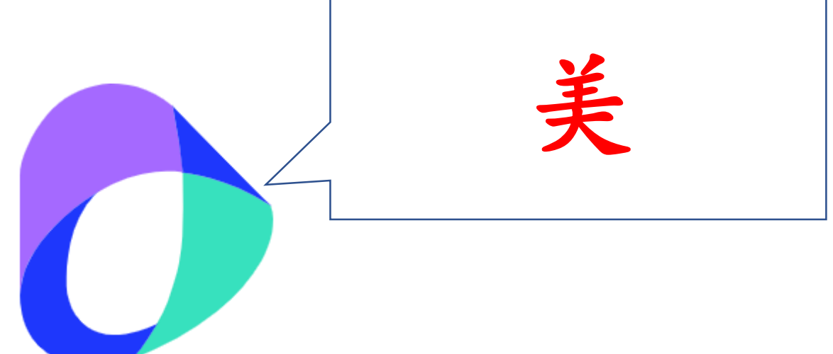
Seed-1.6-VL
