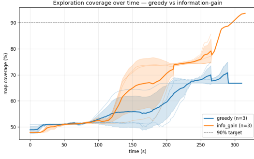
(a) Bonus ( n=3 ) - map coverage over time : information-gain (orange) reaches the 90 % target, greedy (blue) plateaus at \sim 67 –70 %.
