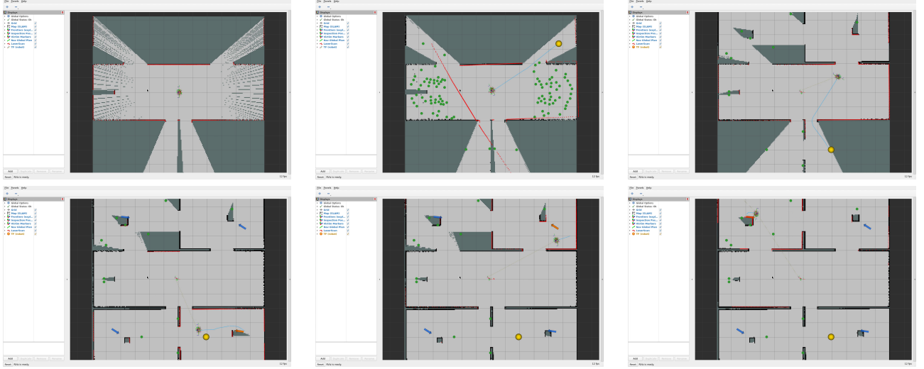
Figure 8: Live RViz at six key moments (1–3: early exploration, map nearly built, phase transition; 4–6: room inspection, victims appearing, final map) - showing the map (SLAM), frontiers, inspection poses, Nav2 plan, LaserScan and the four victim markers. Captured at HD on a virtual X server.
