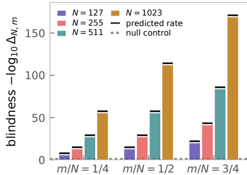
(a) Blindness scaling ( \theta = 0.8 )
