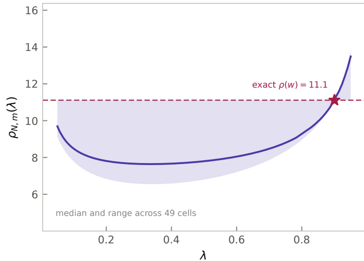
(b) \rho band, \rho(w) = 11.1
