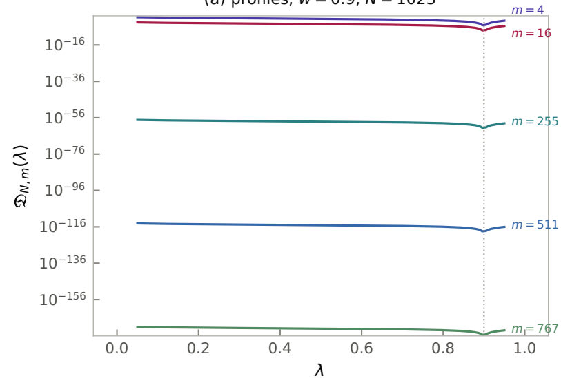
(a) profiles, w = 0.9 , N = 1023
