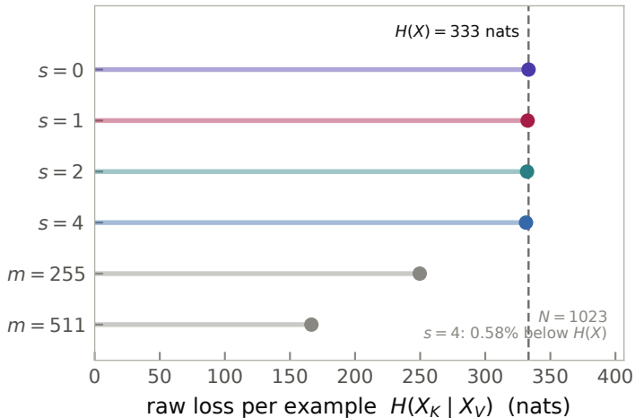
(a) raw loss by mask size
