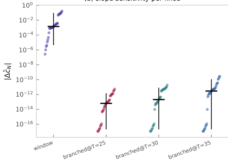
(b) slope sensitivity per knob
