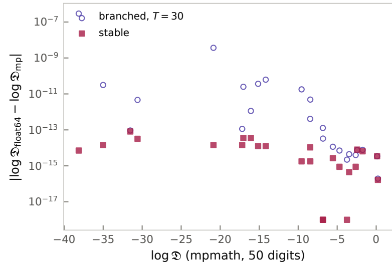
(a) float64 vs mpmath
