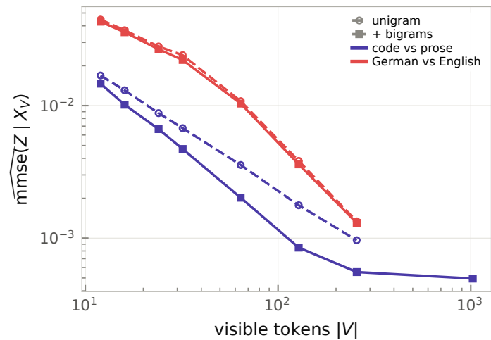
(c) model class: does a richer classifier change the law?
