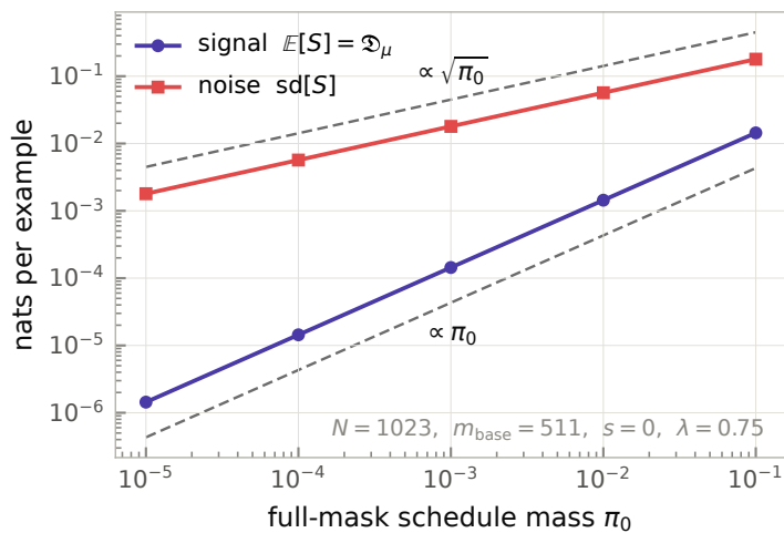
(b) signal grows in \pi_0 , noise only in \sqrt{\pi_0}
