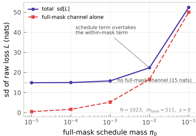
(e) variance of the raw per-example loss
