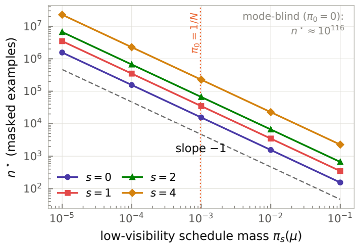
(a) examples needed to detect the discrepancy
