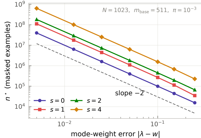
(c) cost of resolving a smaller mode-weight error
