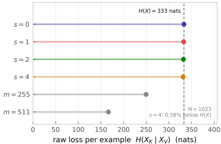
(d) raw loss per example, by mask size
