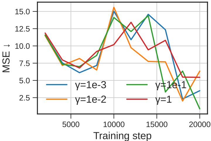
Reconstruction loss vs. \gamma
