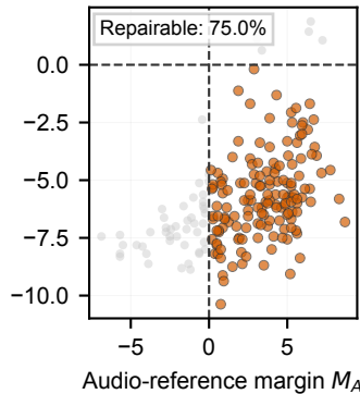
(c) Voxtral-Small-24B x SER
