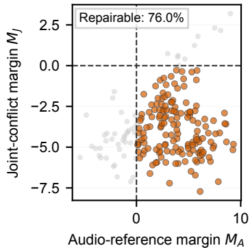
(a) Qwen2-Audio-Inst. x AQA
