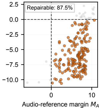
(b) Qwen2.5-Omni x VSC
