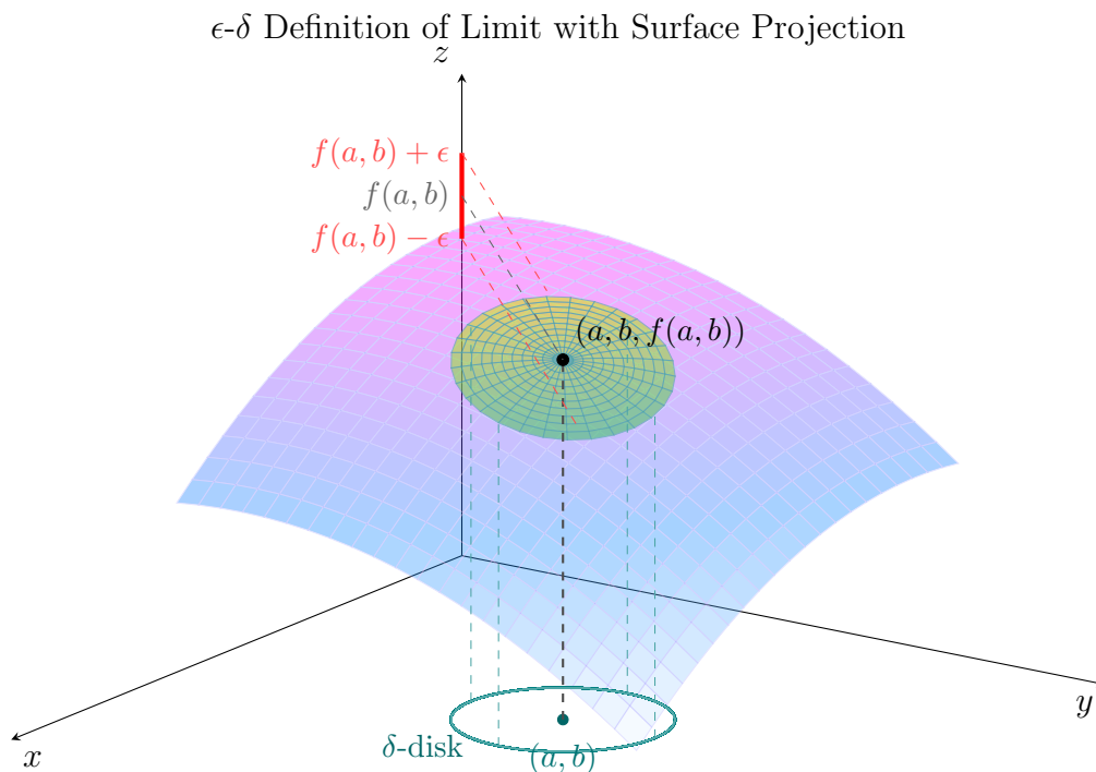
Figure 1: Visualization of the \delta -disk in the xy -plane and its projection onto the surface z = f(x, y) , mapped horizontally to f(a, b) \pm \epsilon on the z -axis.
