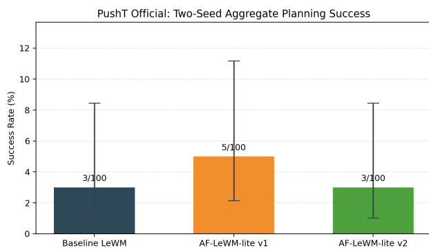
(a) Two-seed planning success with Wilson intervals.
