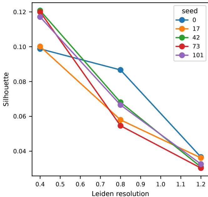
Resolution and seed sensitivity
