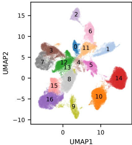
cluster (17 labels)
