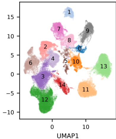
cluster (15 labels)
