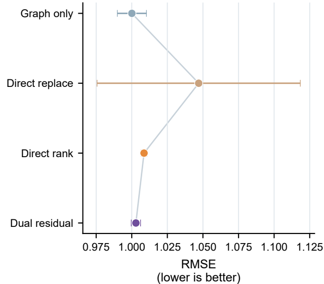
a Point error
