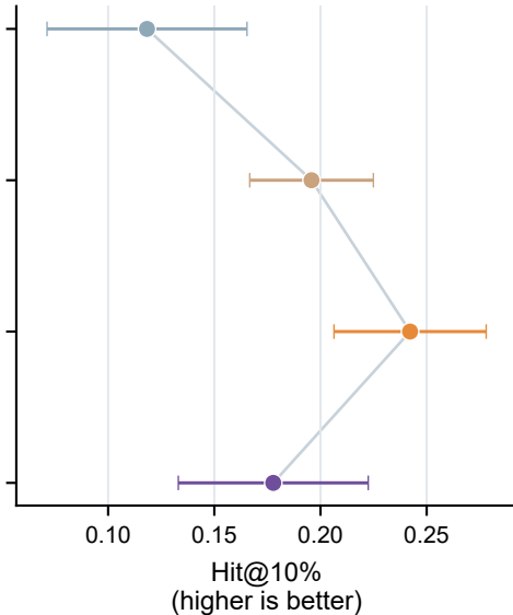
c Top-decile recovery
