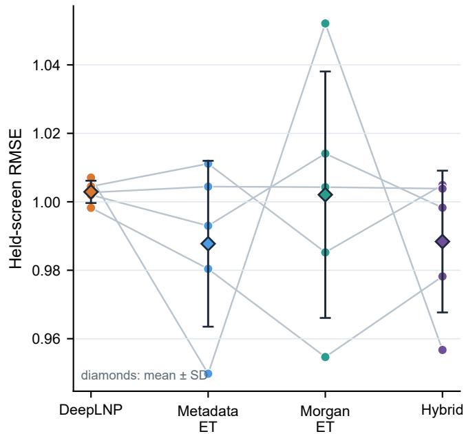
a Paired five-fold point error
