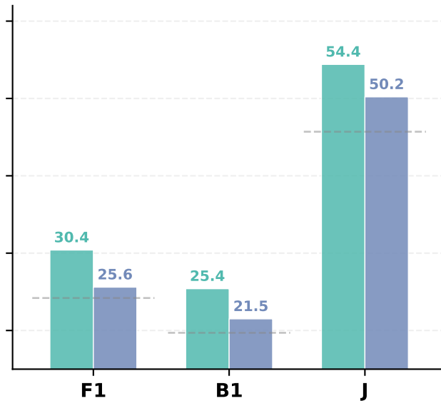
(b) w/o Retrieve Agent RL
