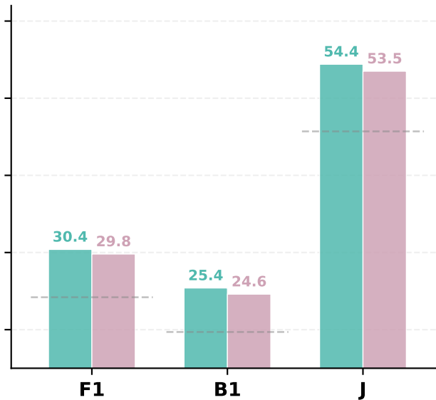
(c) w/o Answer Agent RL
