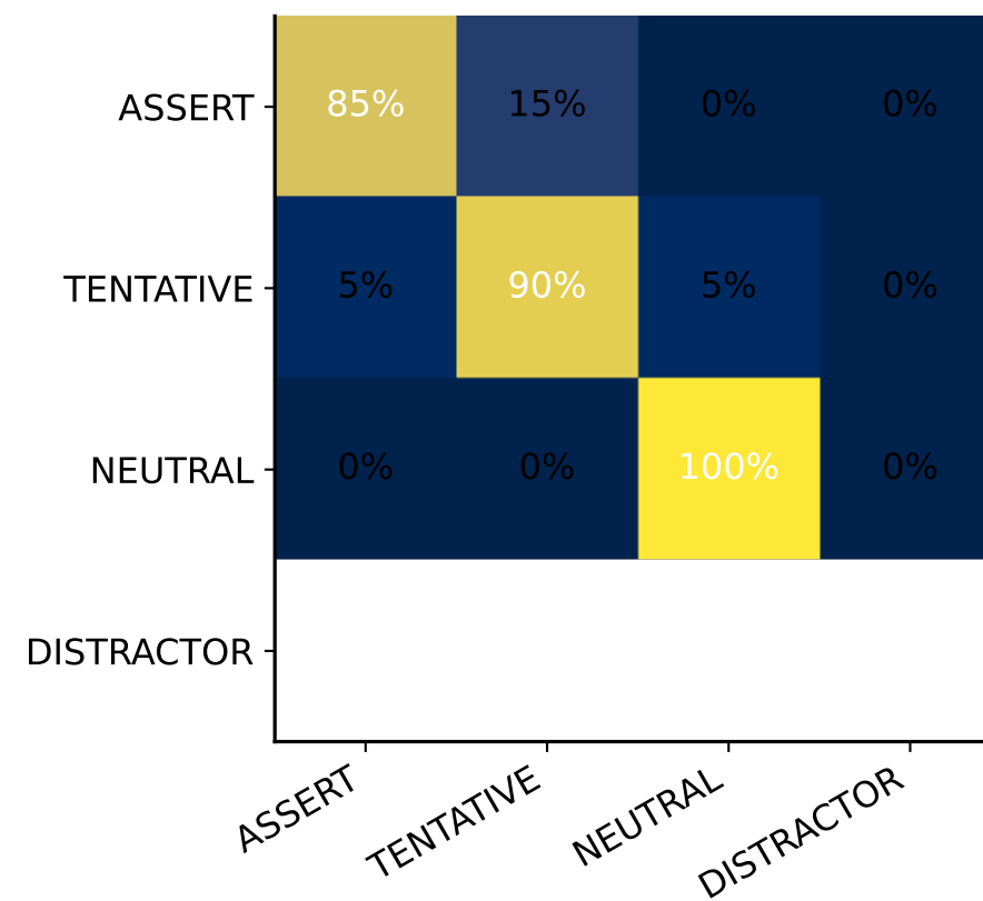
mistral-small-3-24b
