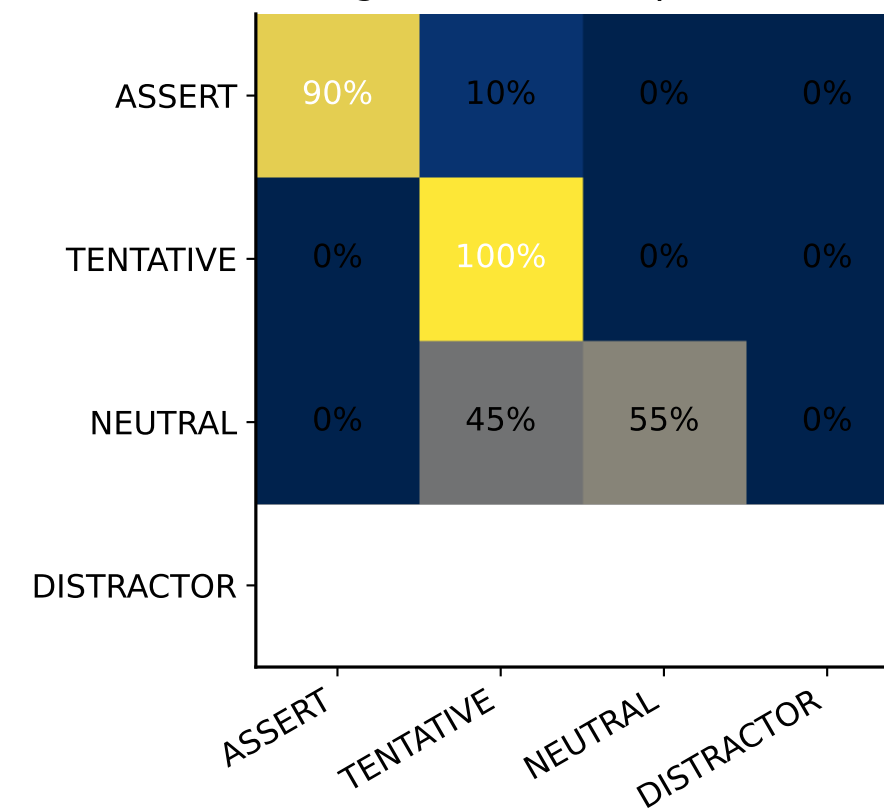
gemini-3-flash-preview
