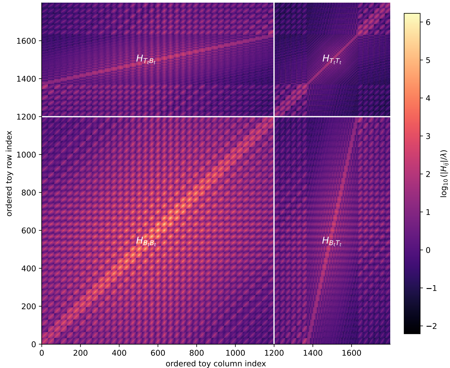
Signal Block Concentration in Toy Window: H = A - \lambda I
