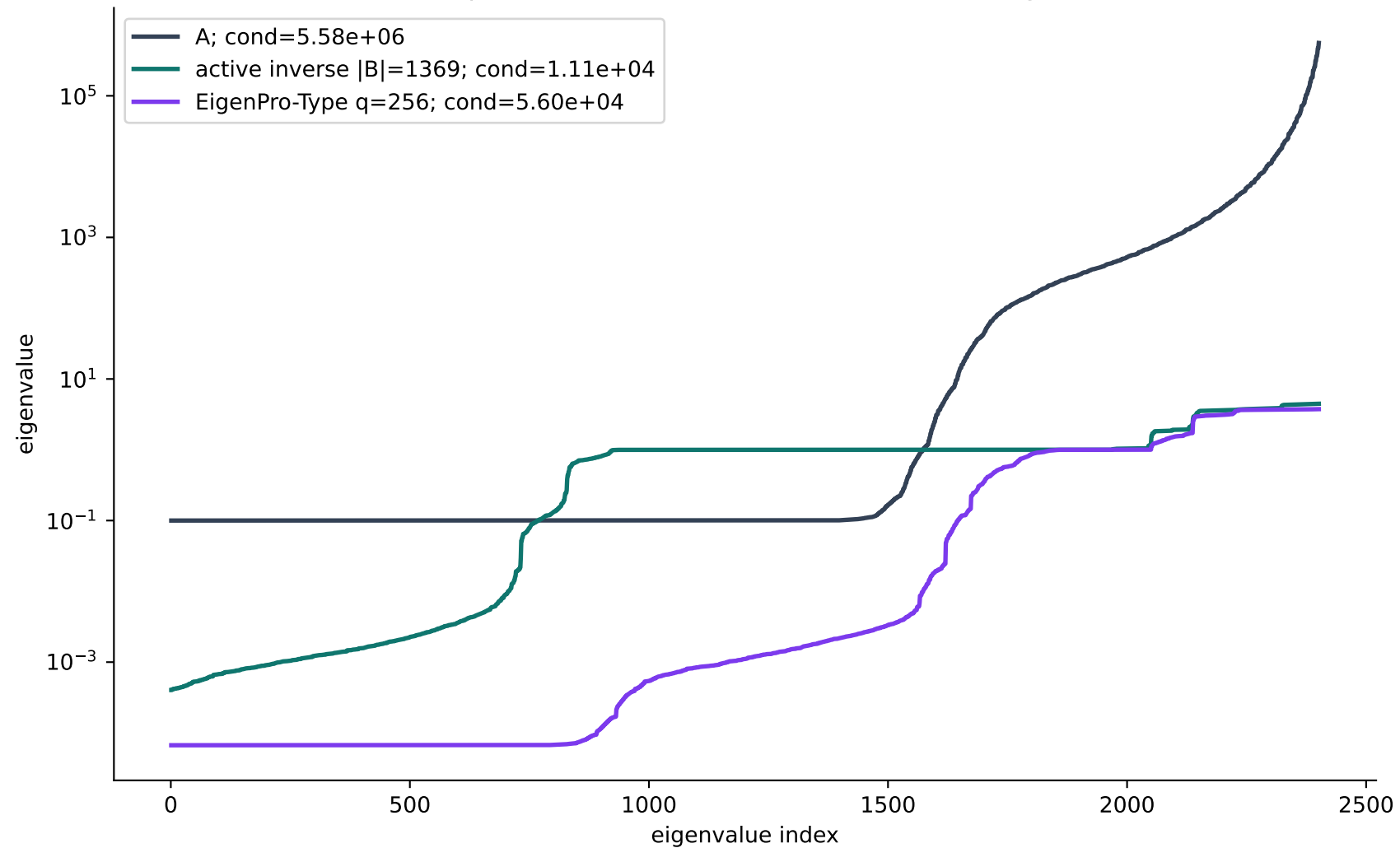
Spectral Effect of Active-Box Preconditioning
