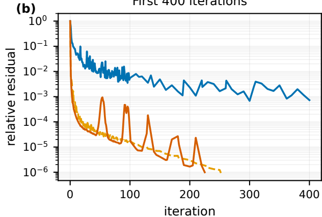
First 400 iterations
