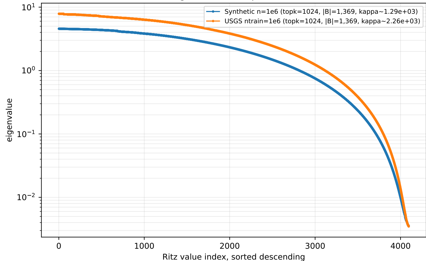
Matern nu=1.5 lengthscale=0.1 spectrum of P^{0.5} A P^{0.5}
