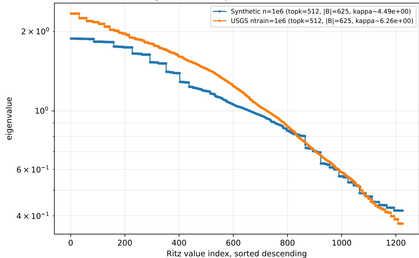
SE lengthscale=0.1 spectrum of P^{0.5} A P^{0.5}
