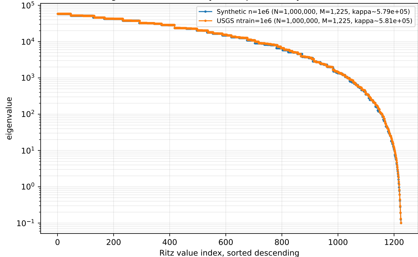
SE lengthscale=0.1 EFGP system spectrum, synthetic vs USGS
