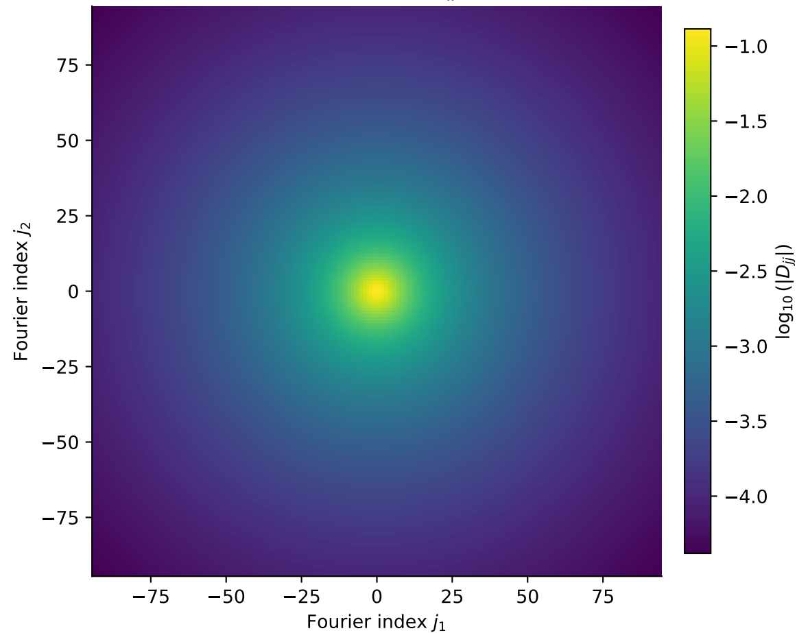
Decrease of |D_{jj}|
