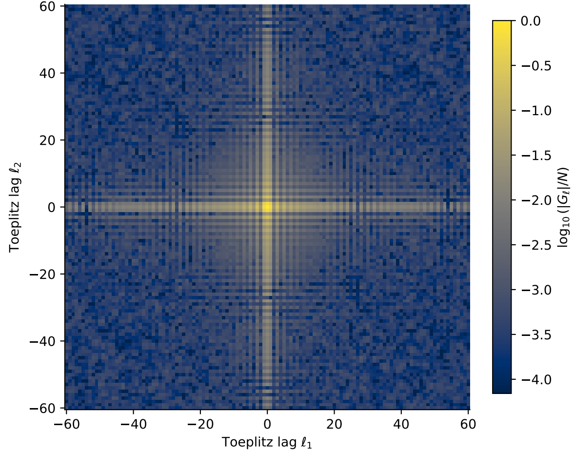
Decrease of |G_\ell|/N for |\ell_i| \leq 60
