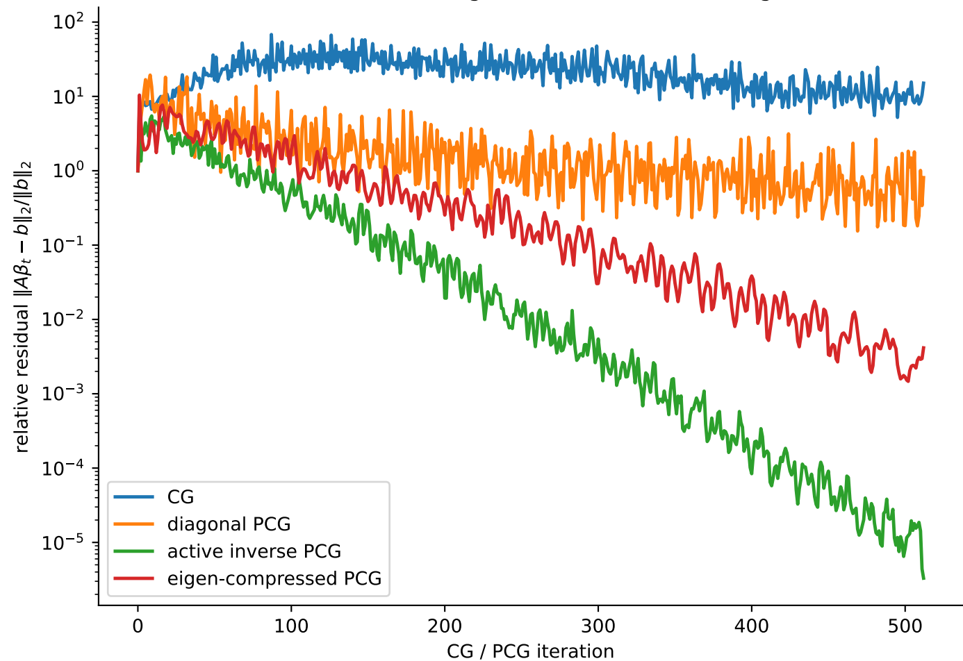
Residual Convergence With Preconditioning
