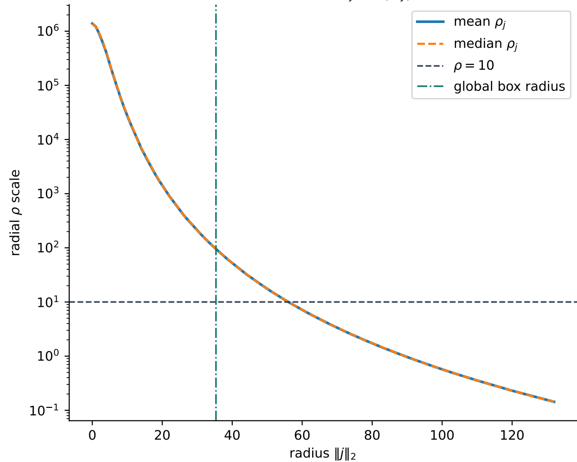
Radial Profile of \rho_j = N|D_j|^2/\lambda
