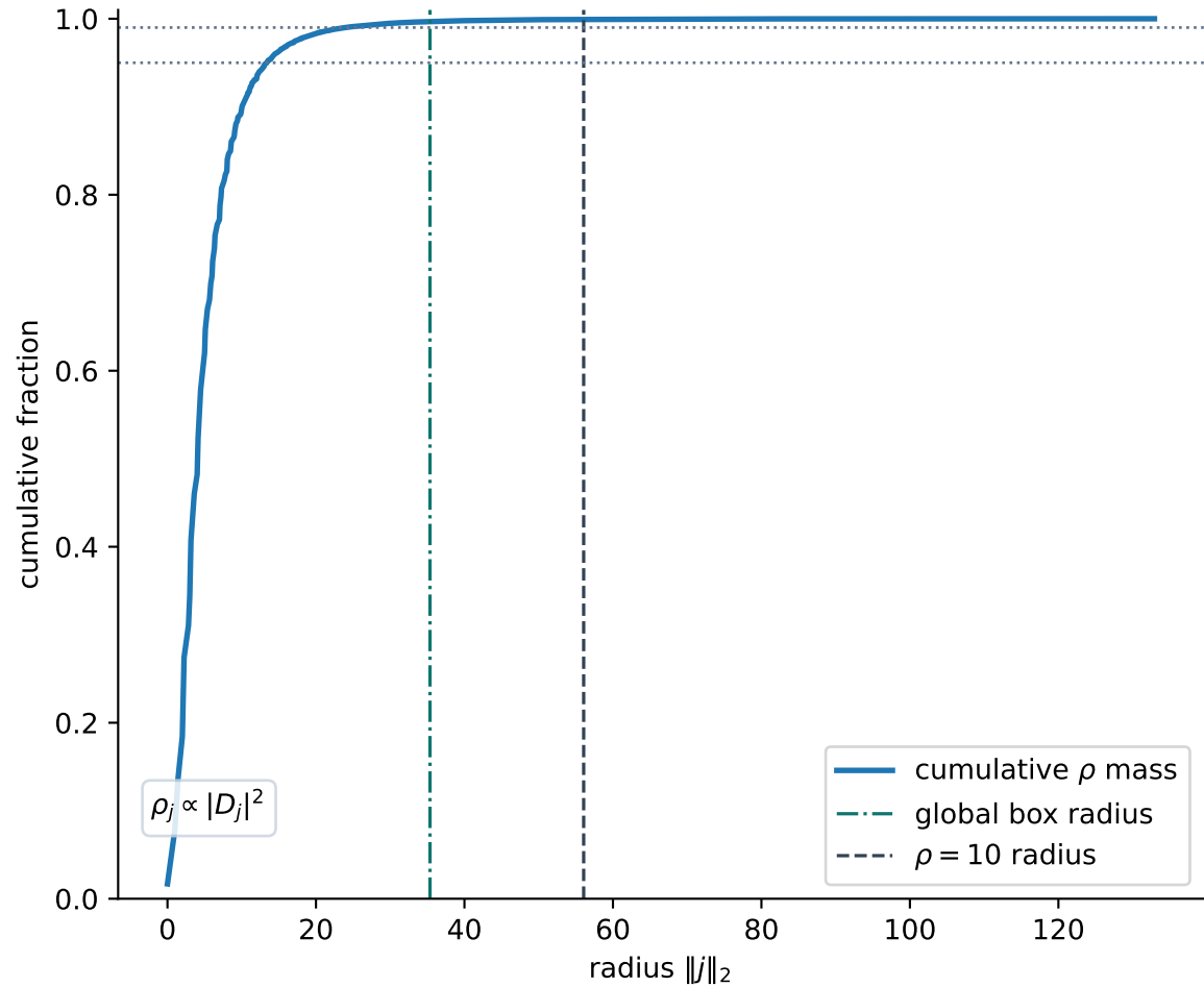
Cumulative \rho Mass (Spectral Mass)
