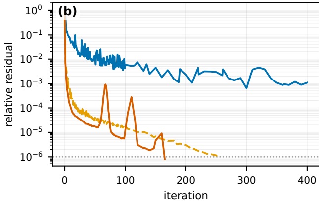
Zoom: first 400 iterations
