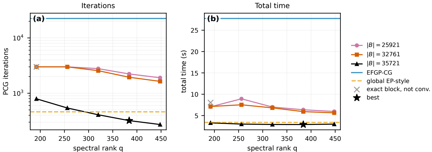
Matern USGS, N = 3 \times 10^8 , M = 35721
