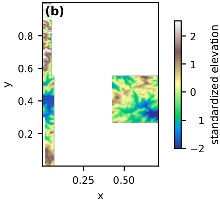
Prediction
