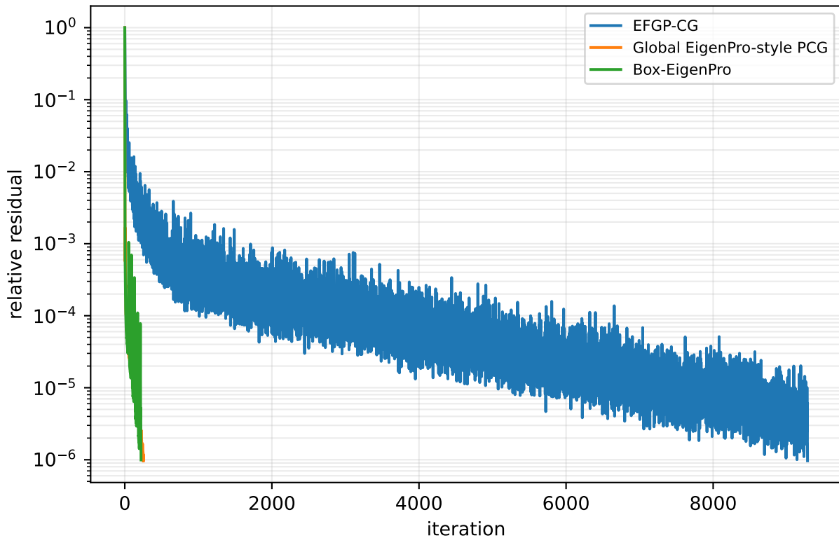
Residual convergence on Matern USGS N=1e8
