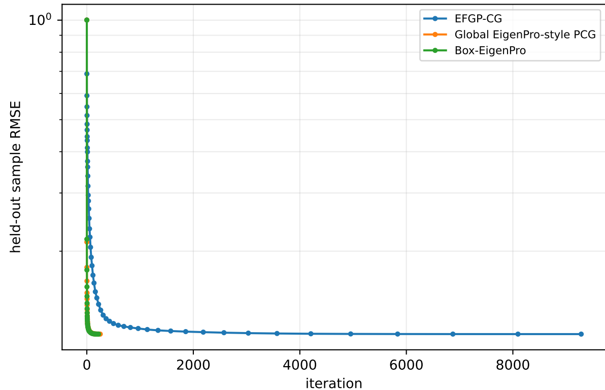
RMSE checkpoints on Matern USGS N=1e8
