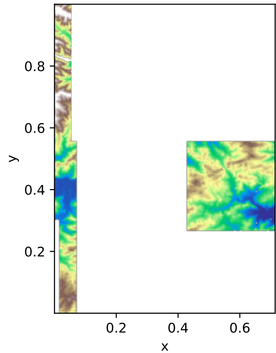
ground truth
