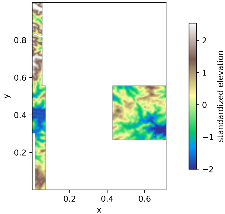
preconditioned prediction
