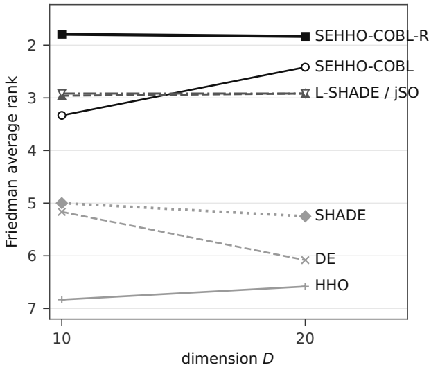
CEC2022, 15,000 evaluations
