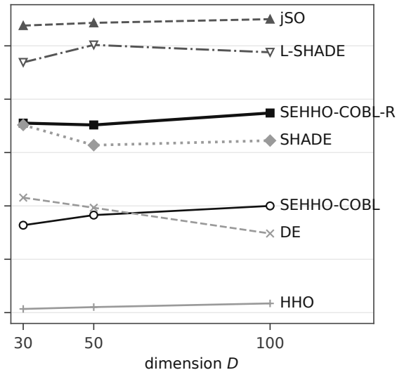
CEC2017, 10,000 \times D evaluations
