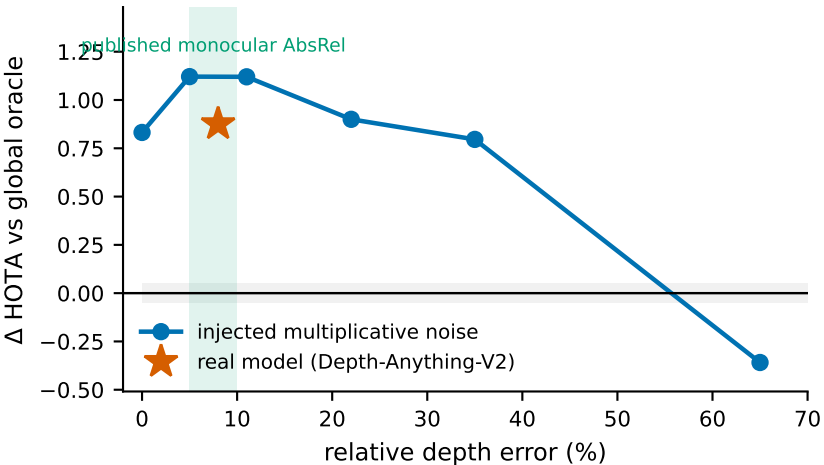
KITTI pedestrians: tolerance to depth error
