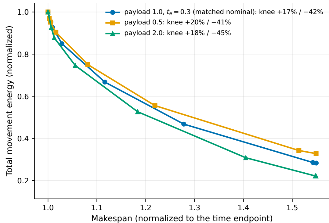
(a) Drone payload coefficient
