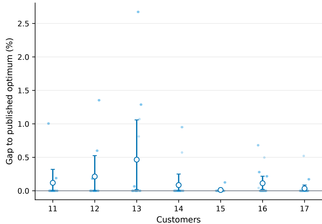
(a) Exact references on small instances
