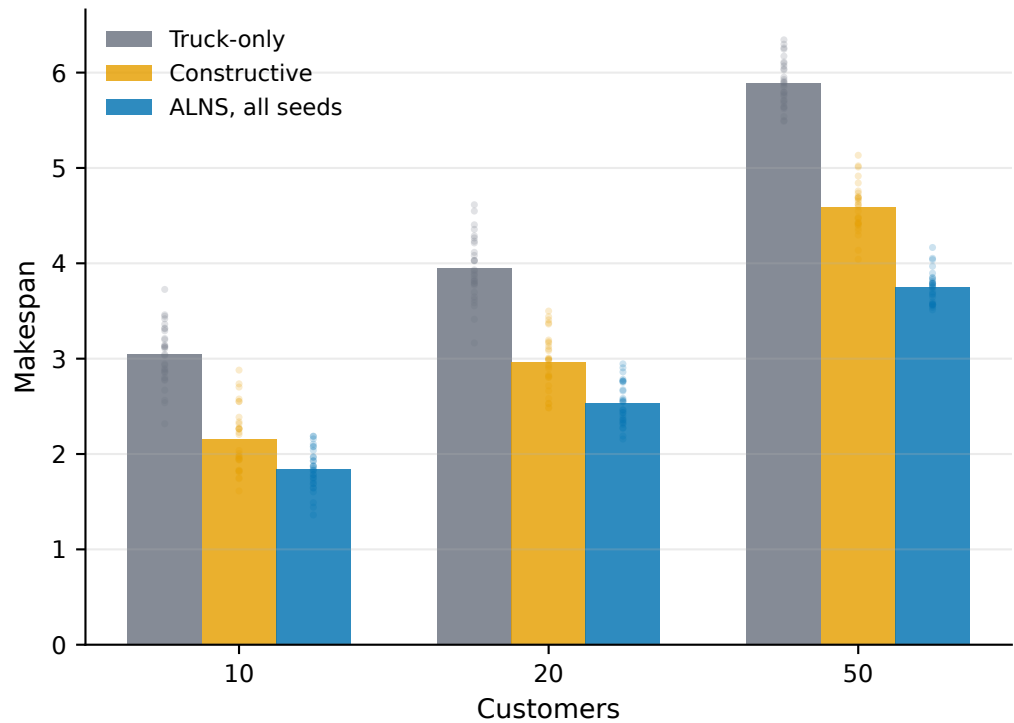
(b) Constructive-reference diagnostics
