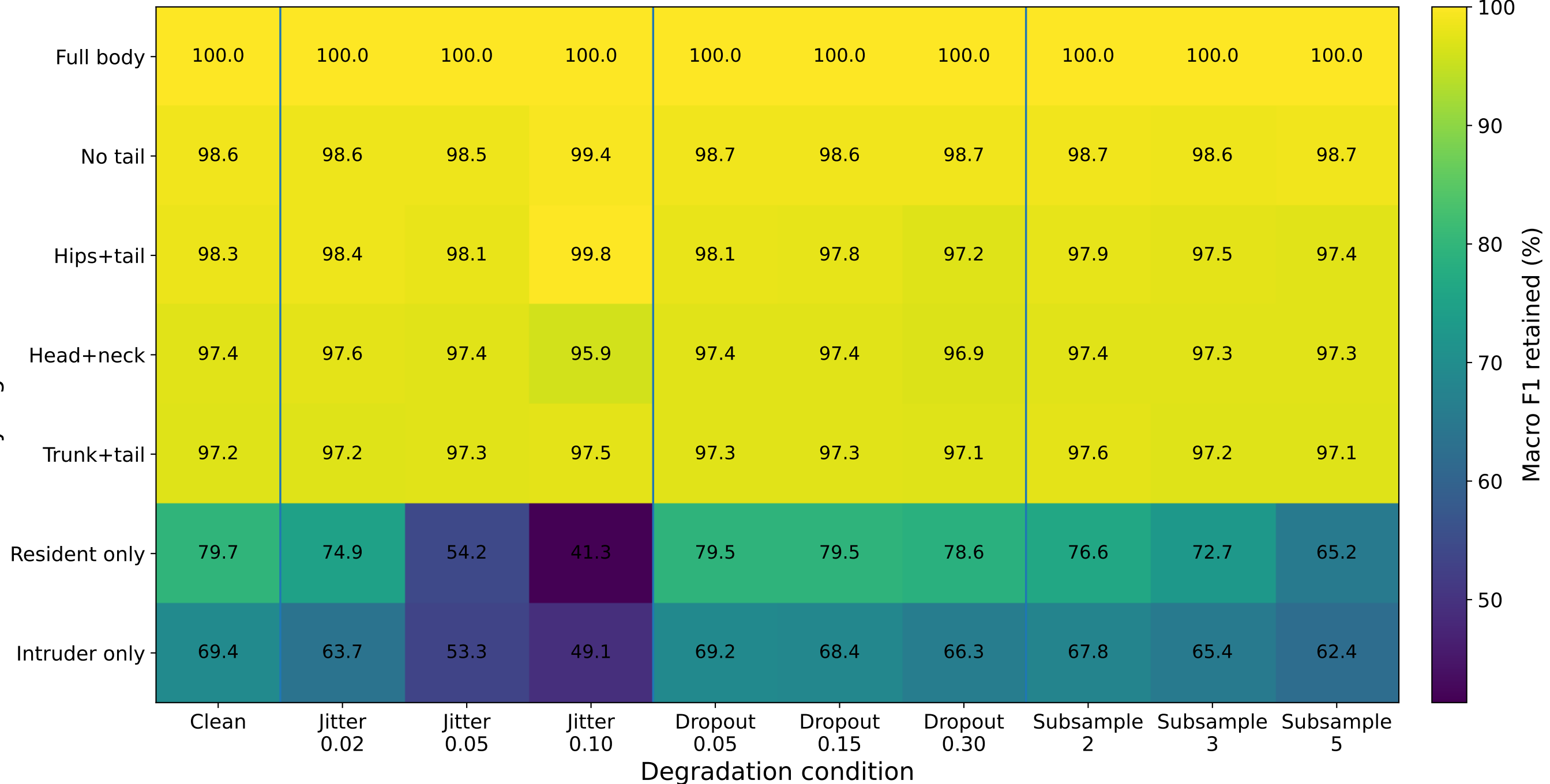
Macro-F1 retention relative to full-body pose under degradation
